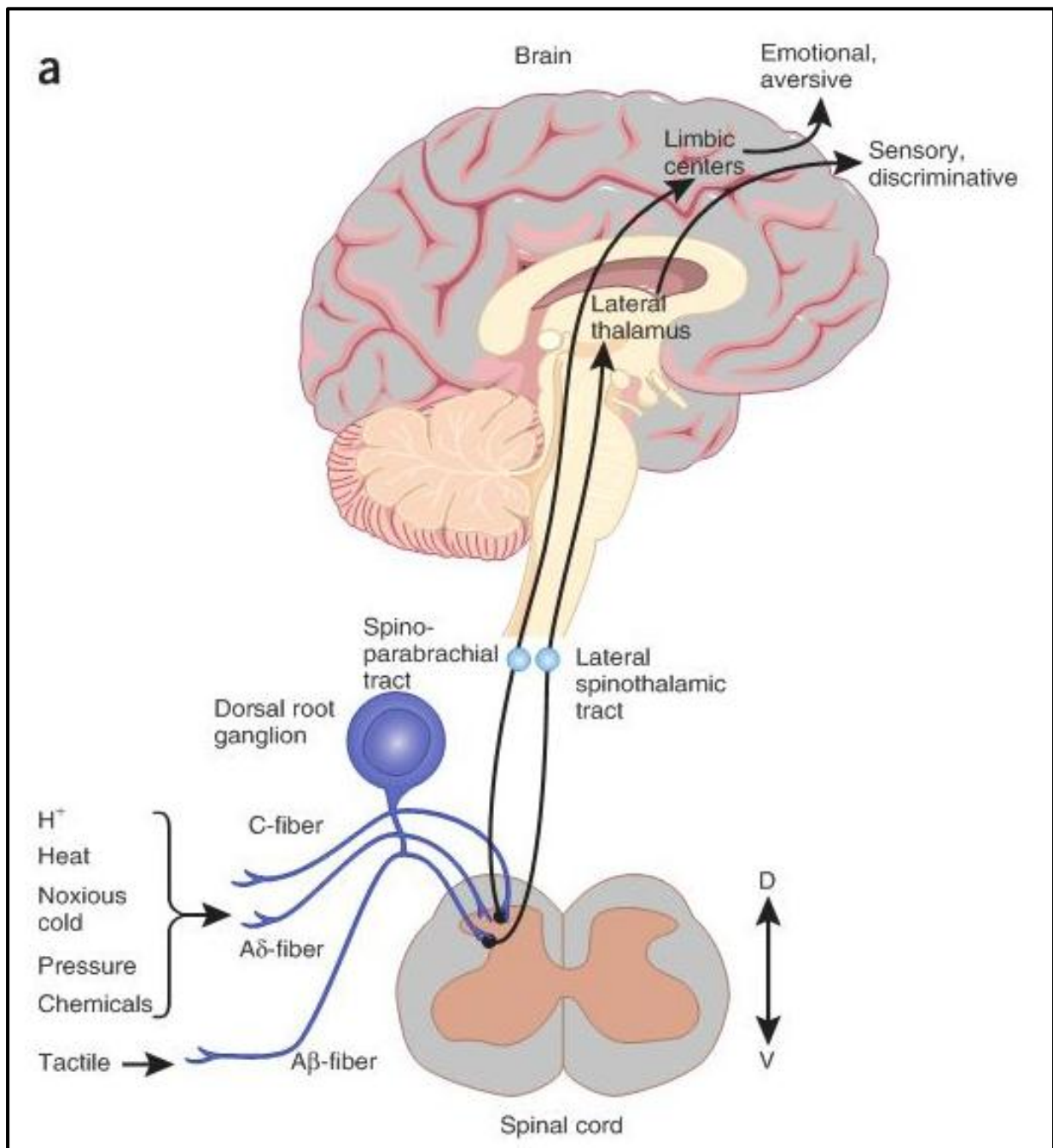
Figure 3.11: A schematic presentation of the circuits that mediate physiological pain
